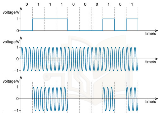
Figure: On/OFF Keying
